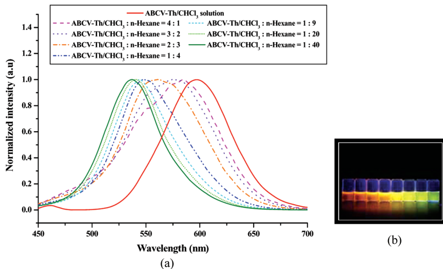
FIGURE 3 (a) Normalized PL spectra of ABCV-Th in various ratio solvents. (b) The fluorescence emission of ABCV-Th ( 1.0 \times 10^{-4} \text{ mol L}^{-1} ) in \text{CHCl}_3 and n-Hexane mixture under the UV light (365 nm). The ratio of \text{CHCl}_3 :n-Hexane from right to left are 1:0, 4:1, 3:2, 2:3, 1:4, 1:9, 1:20, 1:40.
