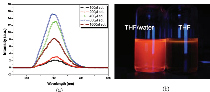
FIGURE 5 (a) Variation of PL spectra of ABCV-Th nanoparticle-suspension (THF/water) with the concentration of ABCV-Th, in which the injected ABCV-Th solution ( 1.0 \times 10^{-4} \text{ M} in THF) were 100 \mu\text{l} , 200 \mu\text{l} , 400 \mu\text{l} , 800 \mu\text{l} and 1600 \mu\text{l} . (b) The fluorescence emission of ABCV-Th nanoparticles suspension in THF/water and THF with irradiation of UV-light (365 nm).
